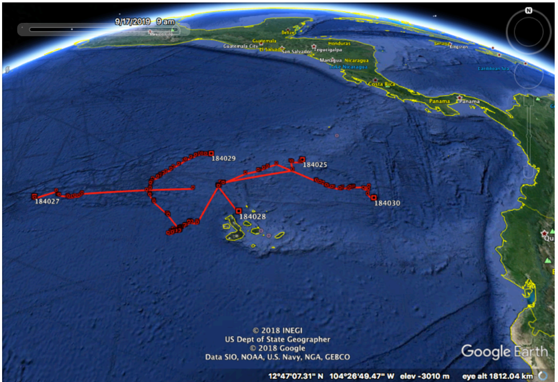
Figure 26: Tracks of the 5 SPOT6 tags since the date of tagging giving regional perspective (see Appendix #1).
